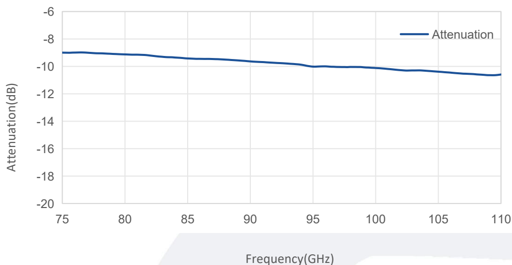
Attenuation vs Frequency
