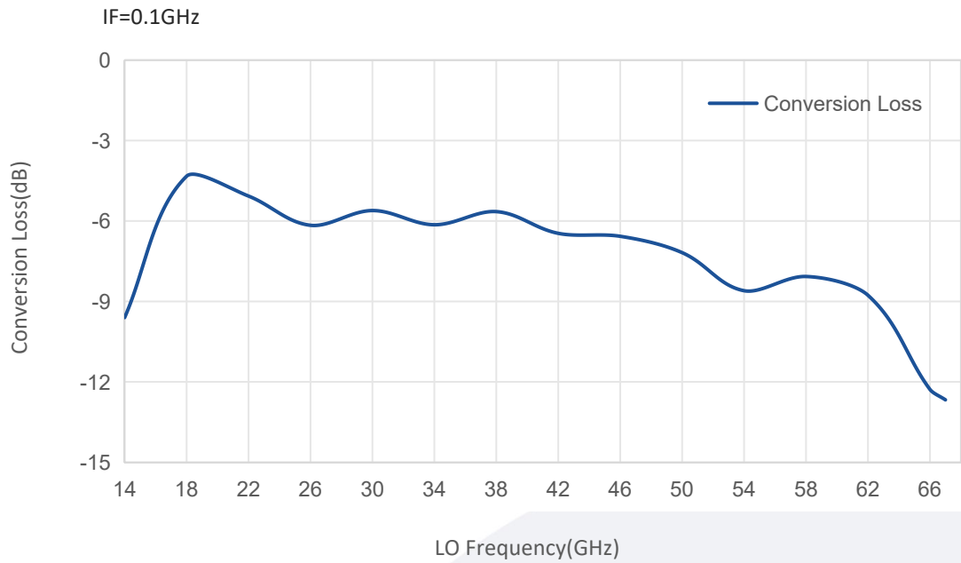
Coverison Loss vs LO Frequency
