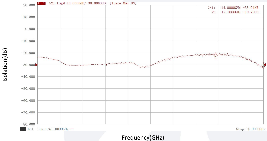
RF to Q Isolation vs Frequency
