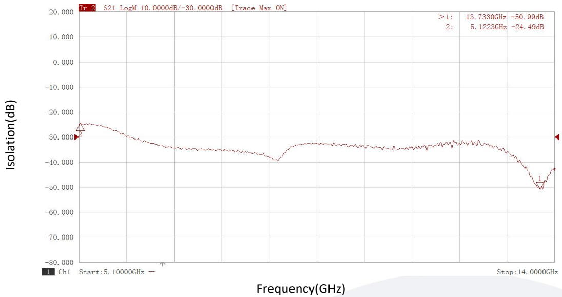
RF to I Isolation vs Frequency
