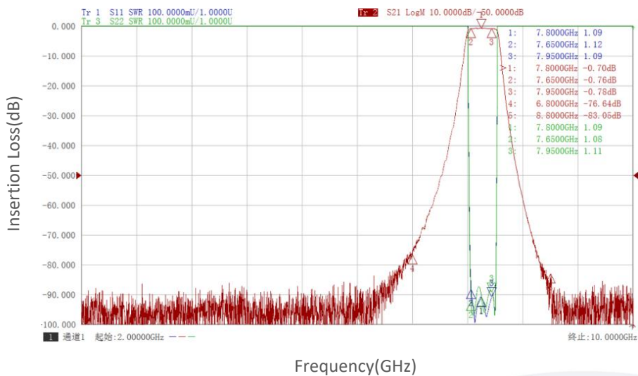
Insertion Loss vs Frequency
