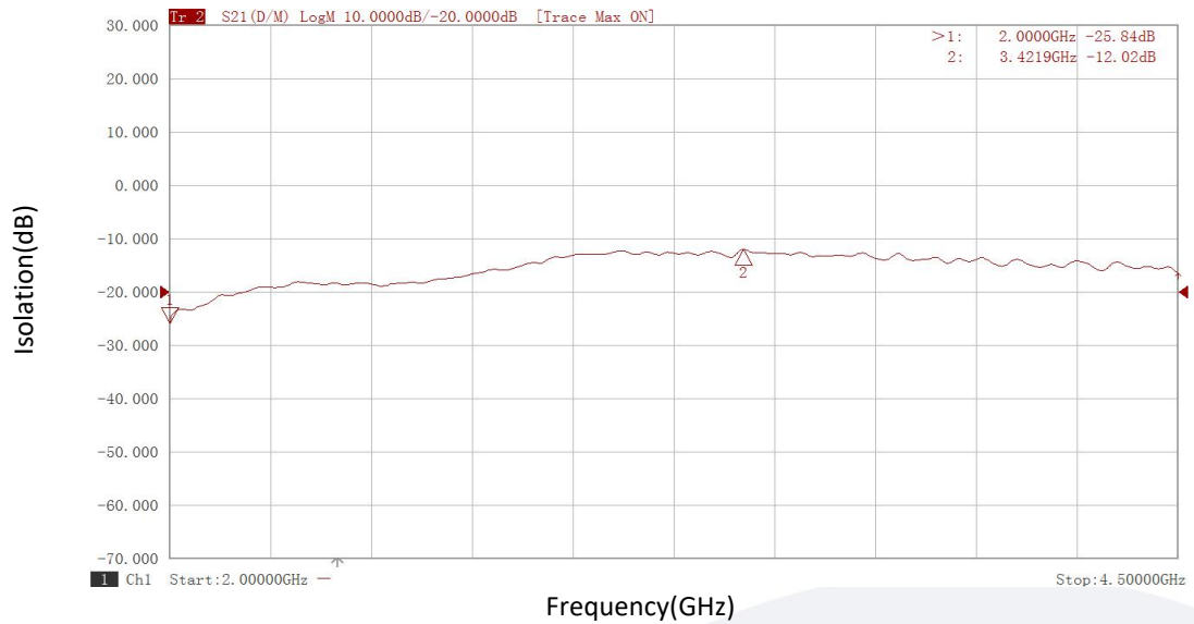
LO to IF1 Isolation vs Frequency
