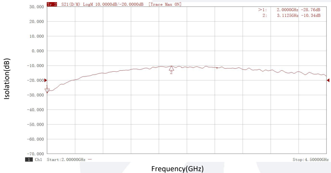
LO to IF2 Isolation vs Frequency
