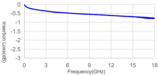
A81-NWMNWM-1m Insertion Loss
