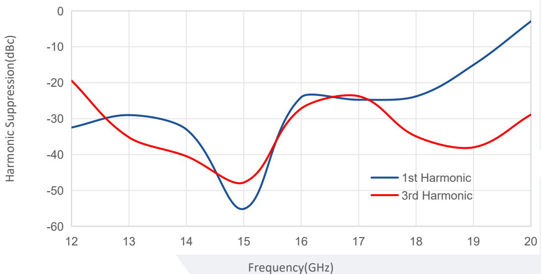
Harmonic Suppression vs Frequency
