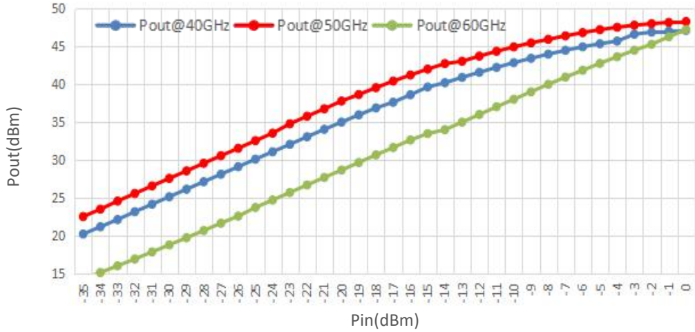
Pout@Equal_Pin
