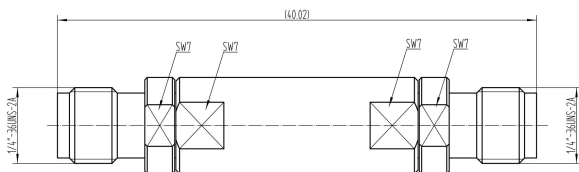
TLLF-DC-3G-FF
