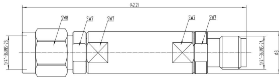
TLLF-DC-3G-K
