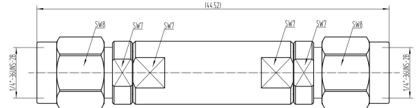
TLLF-DC-3G-MM
