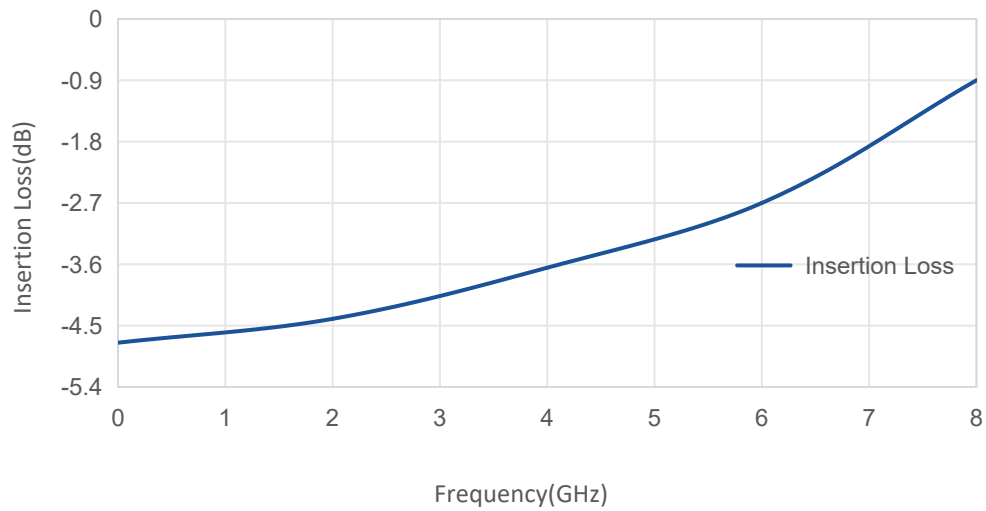
Insertion Loss vs Frequency
