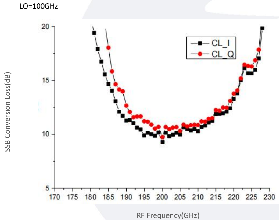
SSB Conversion Loss vs RF Frequency
