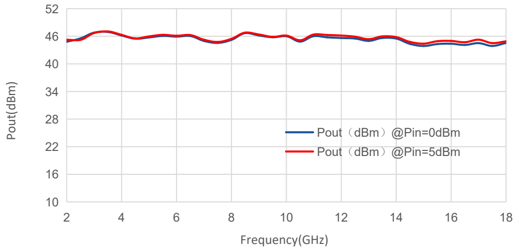
Pin@Psat vs Frequency
