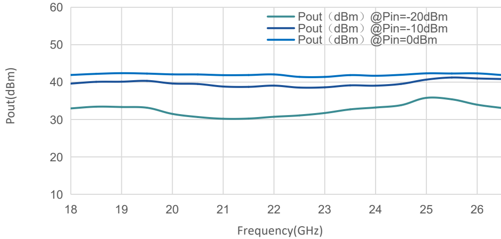
Pin@Pout vs Frequency
