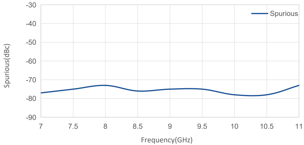
Spurious@Pout=57dBm
