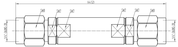
TLHF-8G30G-MM
