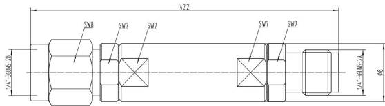
TLHF-8G30G-K
