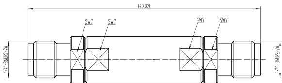
TLHF-6G30G-FF
