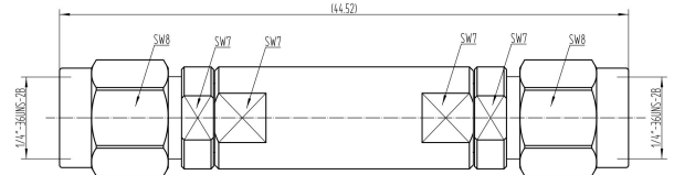
TLHF-6G30G-MM
