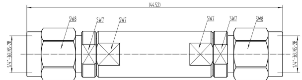
TLHF-5G26G-MM
