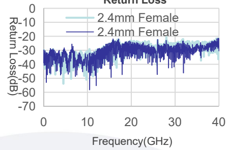
A40-2.4M2.4F-1m Return Loss
