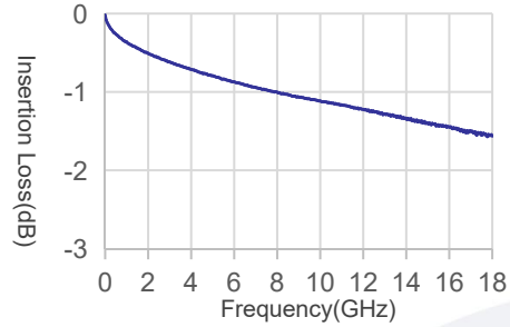
A40-SMAMSMAWM-1m INSERTION LOSS
