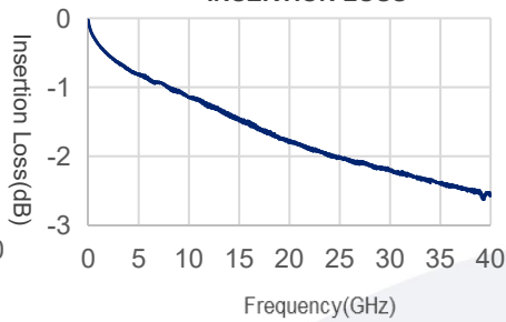
A40-2.92WM2.92WM-1m INSERTION LOSS
