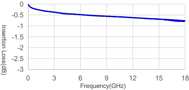
A81-SMAMFSMAF-1m Insertion Loss
