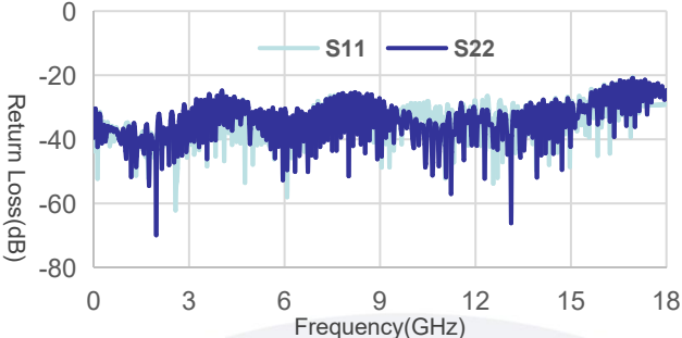
A81-SMAFSMAF-1m Return Loss
