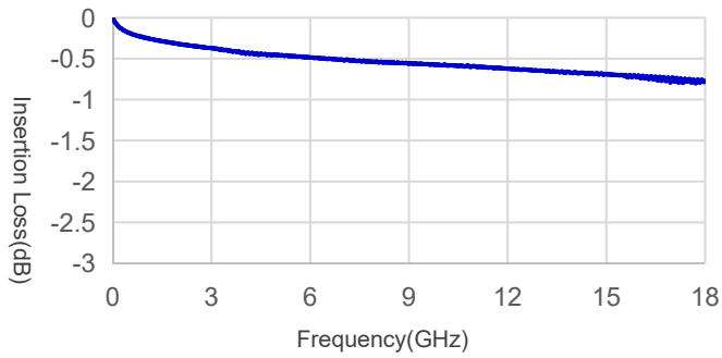
A81-NMNF-1m Insertion Loss
