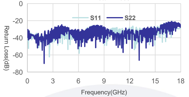
A81-NWMNWM-1m Return Loss
