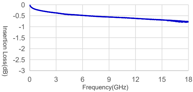
A81-NWMNWM-1m Insertion Loss
