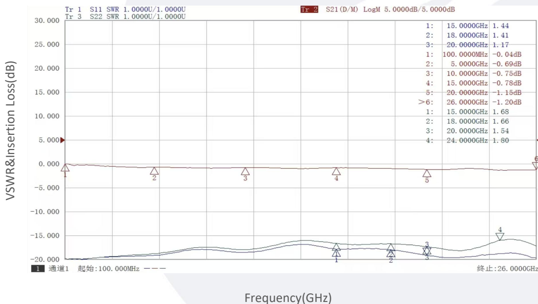
VSWR&Insertion Loss vs Frequency
