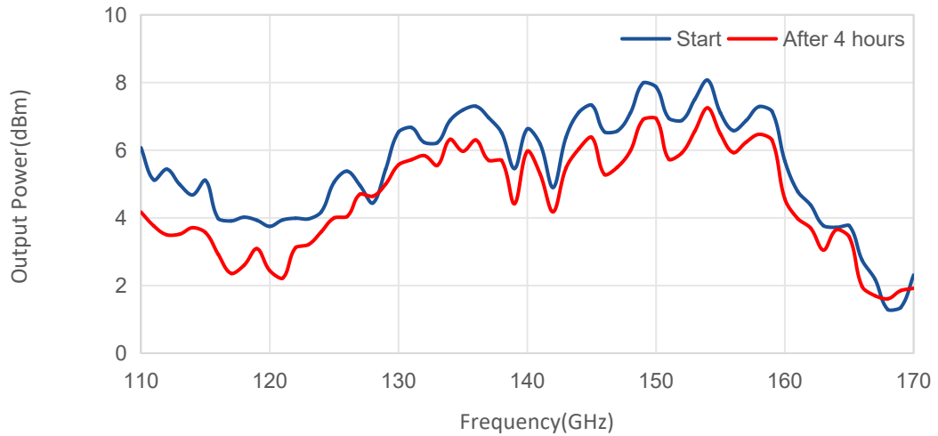
Output Power Stability vs Frequency
