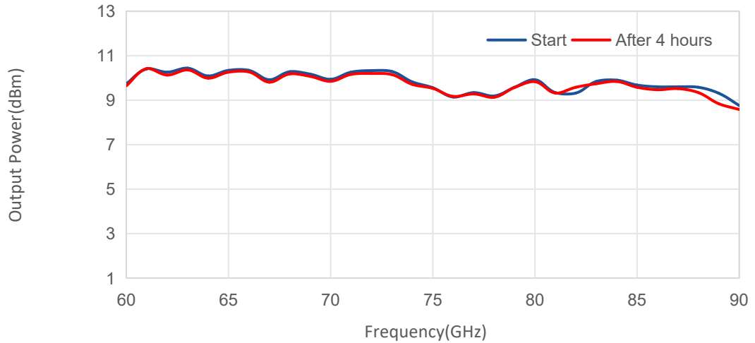
Output Power Stability vs Frequency
