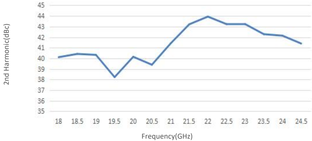
2nd Harmonic vs Frequency
