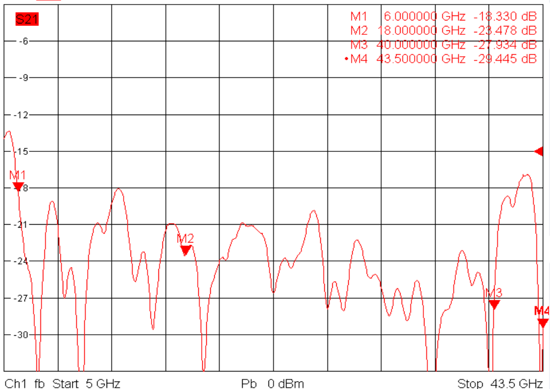
Trc1 S21 dB Mag 3 dB / Ref -15 dB Cal 1
