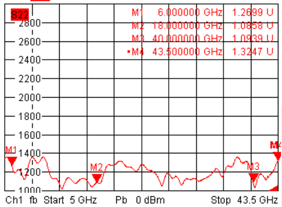
Trc4 S22 SWR 200 mU / Ref 1 U Cal 4
