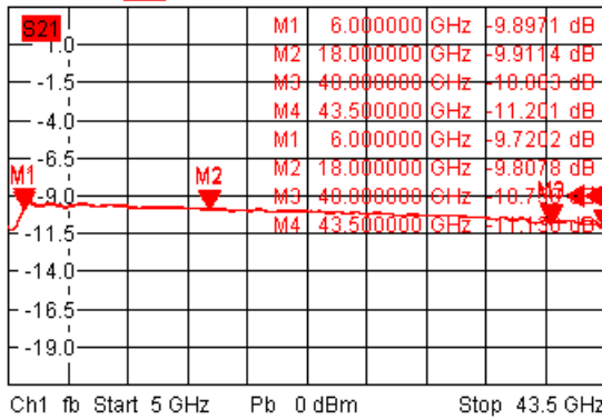
Trc3 S21 dB Mag 2.5 dB / Ref -9 dB Cal 3 Mem[Trc3] S21 dB Mag 2.5 dB / Ref -9 dB
