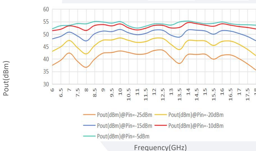
Pout@Equal_Pin
