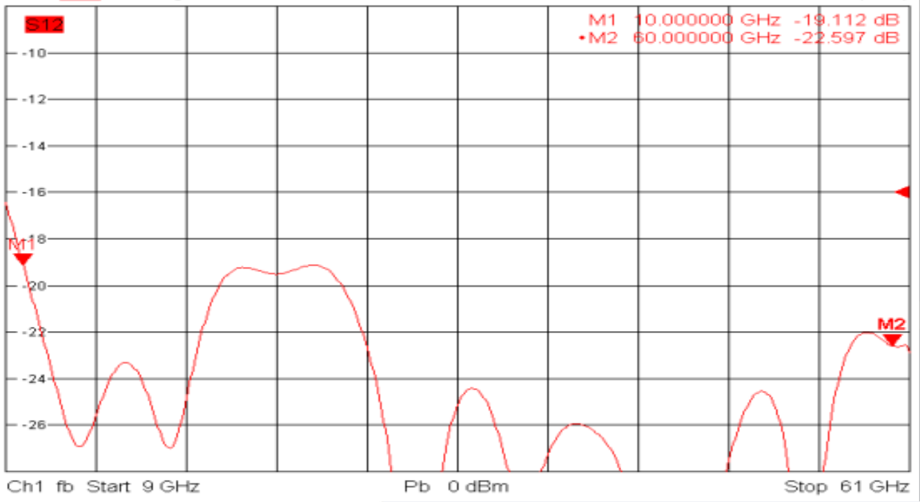
Trc2 S12 dB Mag 2 dB / Ref -16 dB Cal
