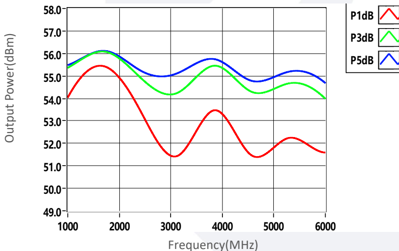
Output Power vs Frequency
