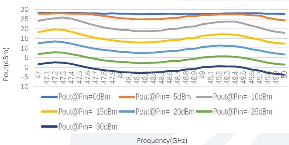
Pout@Equal_Pin
