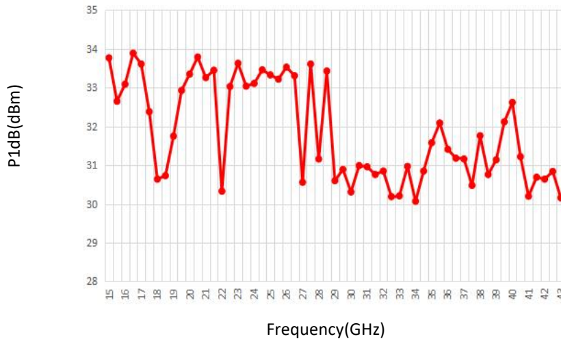
Spurious@Pout=30dBm
