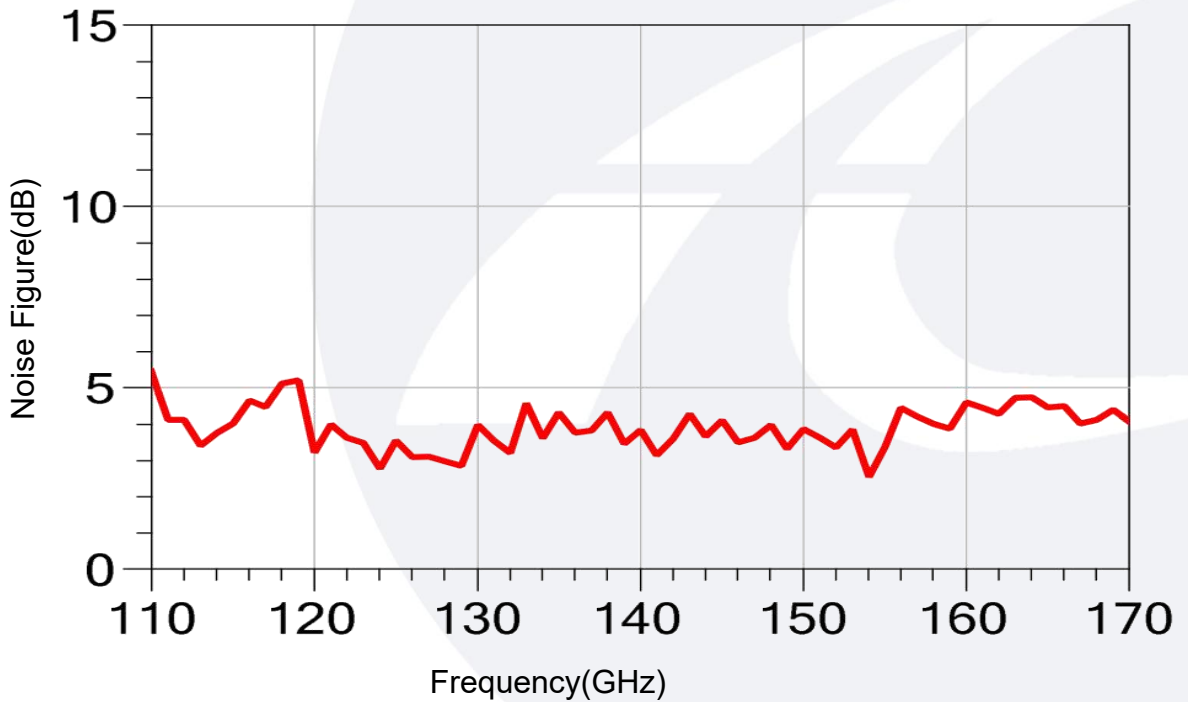
Noise Figure vs Frequency
