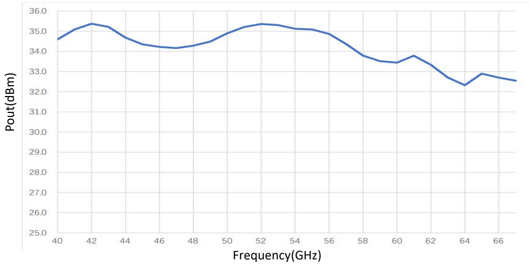
Pout vs Frequency
