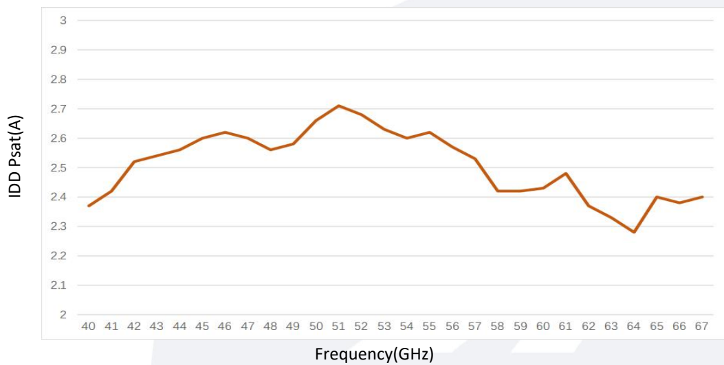
IDD Psat vs Frequency
