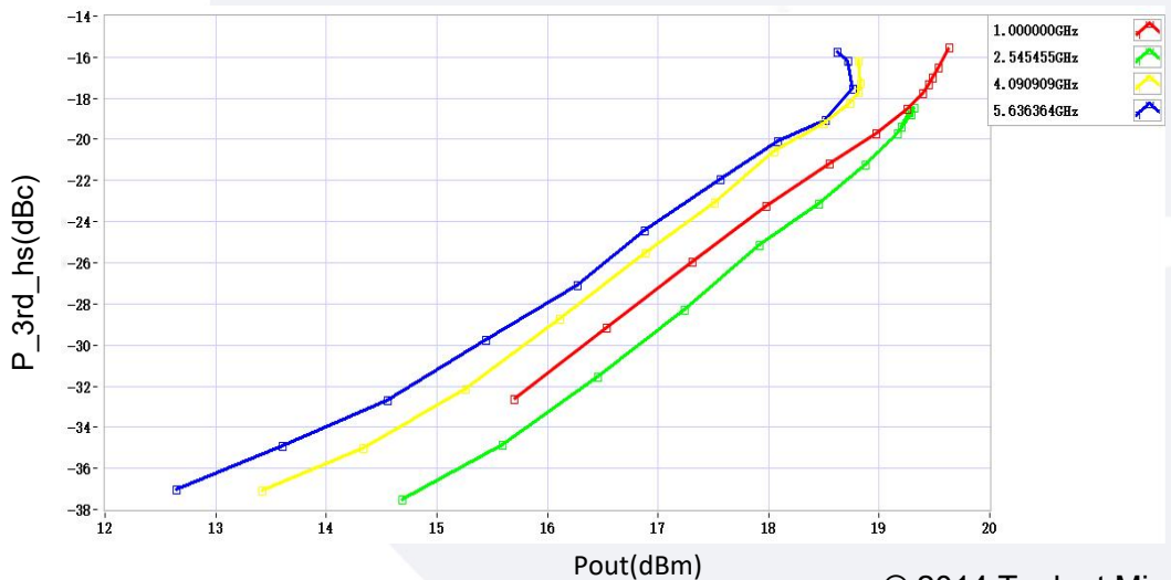
3rd Harmonic (dB) vs Output Power
