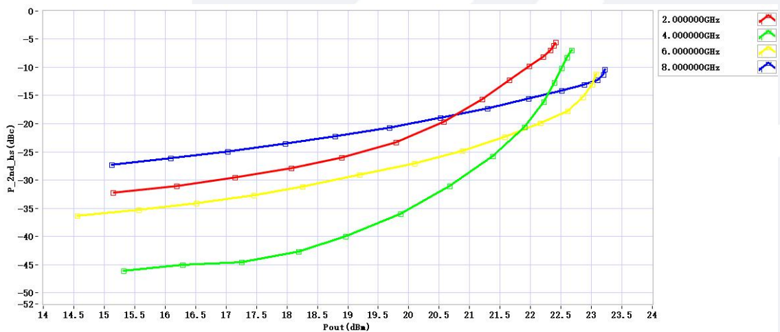
2nd Harmonic(dBc) vs. Output Power
