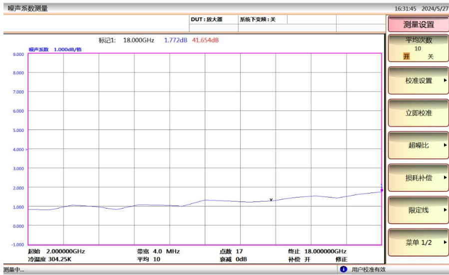
Noise Figure vs Frequency
