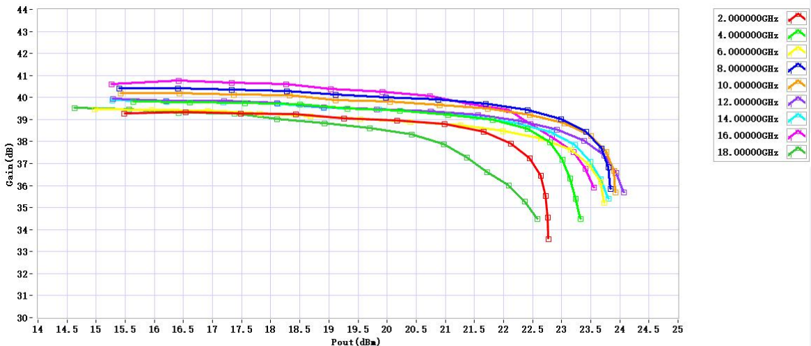
Gain vs Output Power
