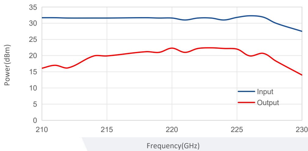
Input&Output Power vs Frequency
