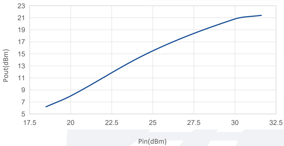
Pout vs Pin
