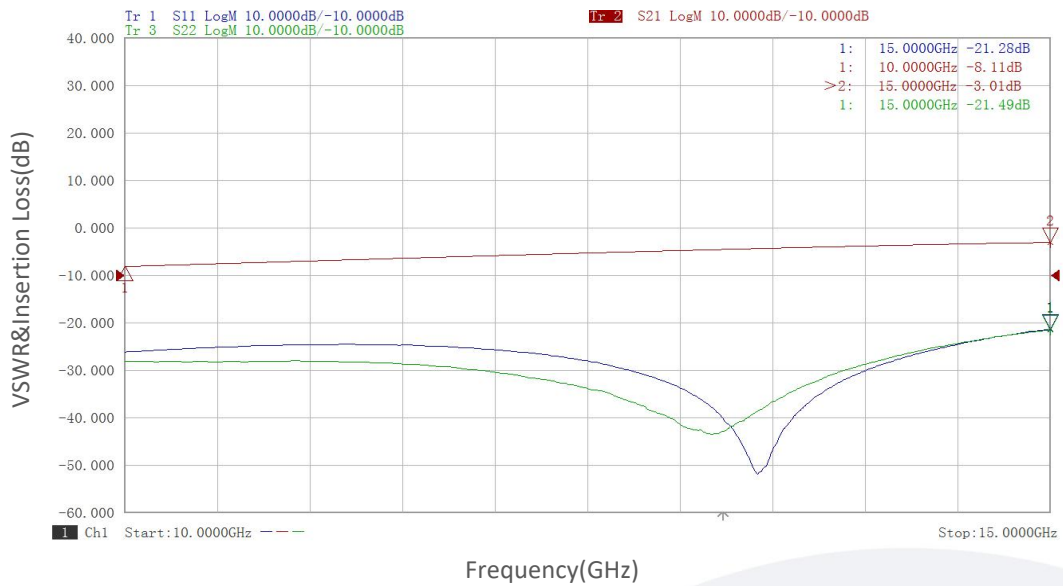
VSWR&Insertion Loss vs Frequency
