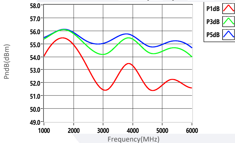
PndB vs Frequency
