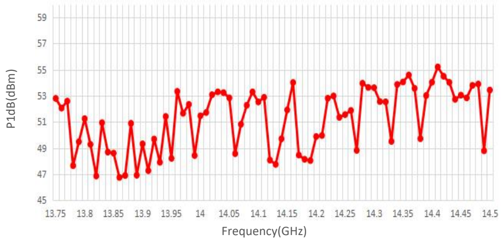
Pin@@Equal_Pout
