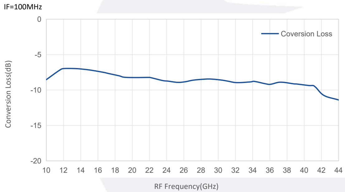
Coverison Loss vs RF Frequency
