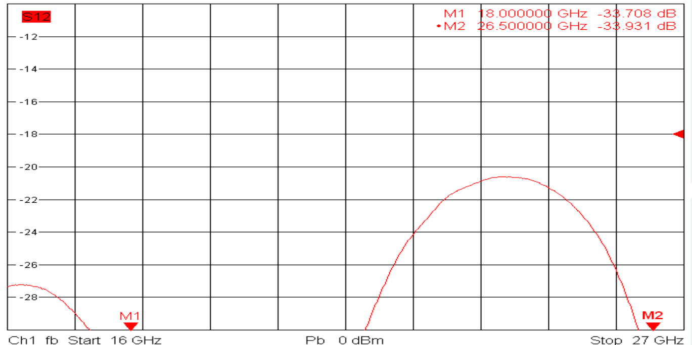
Trc2 S12 dB Mag 2 dB / Ref -18 dB Cal
