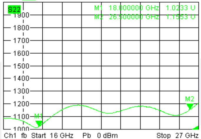
Trc4 S22 SWR 100 mU/ Ref1 U Cal 4
