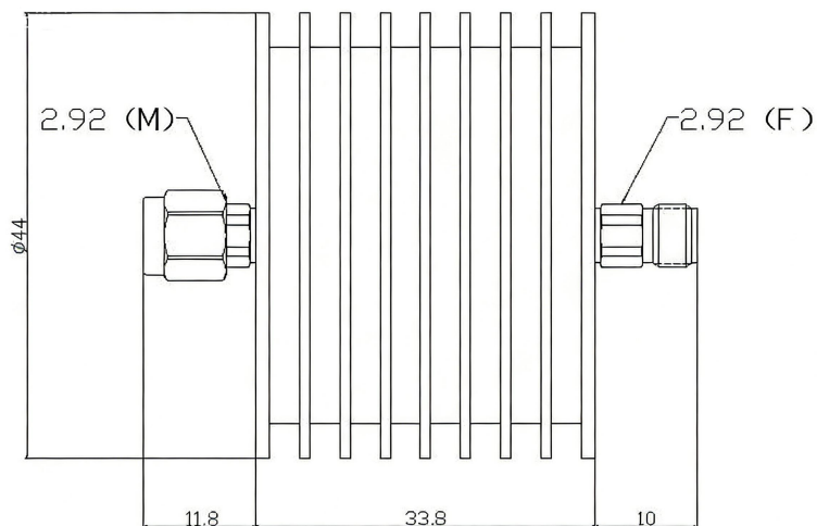
3-30dB Outline dimensions
