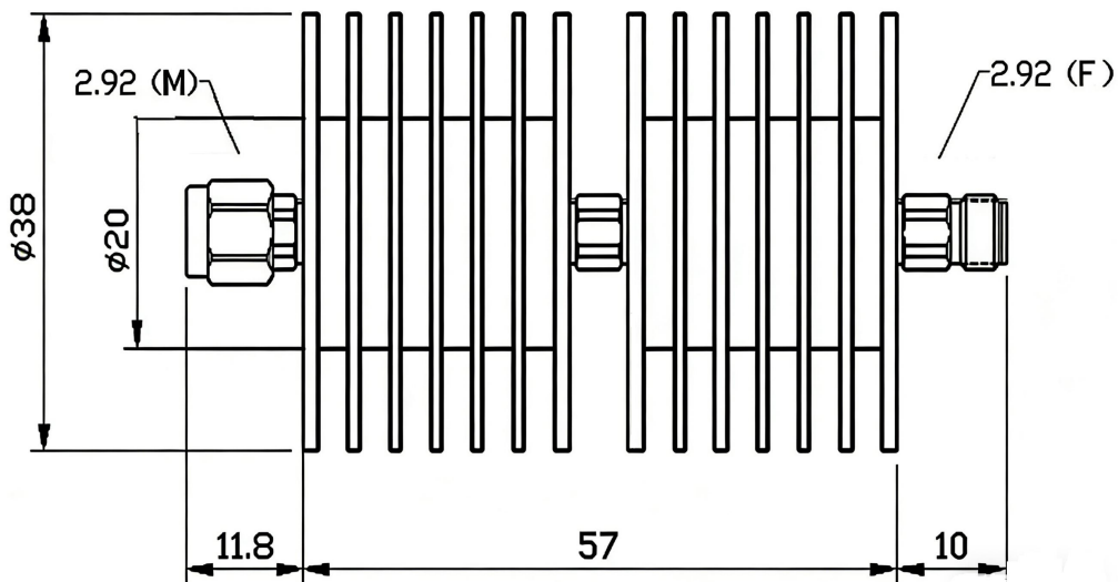
40dB Outline dimensions
