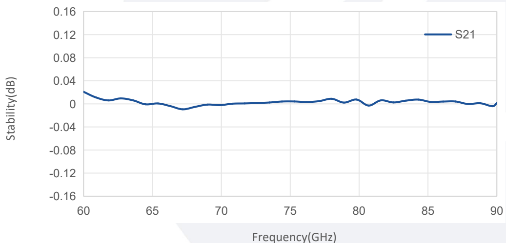
Stability@2h vs Frequency
