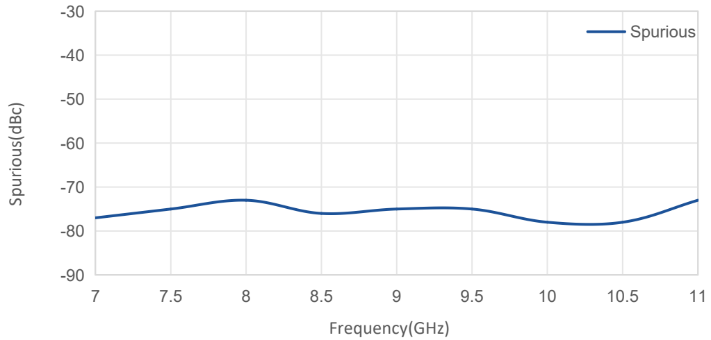
Spurious@Pout=57dBm
