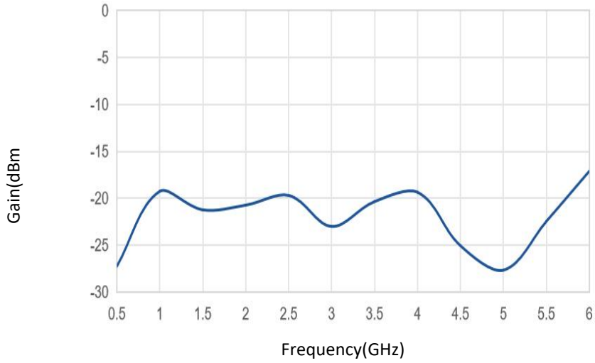
P1dB VS Frequency
